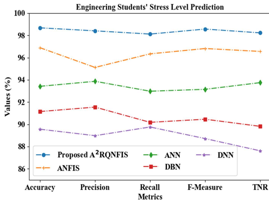
Figure 4: Performance estimation based on performance metrics
