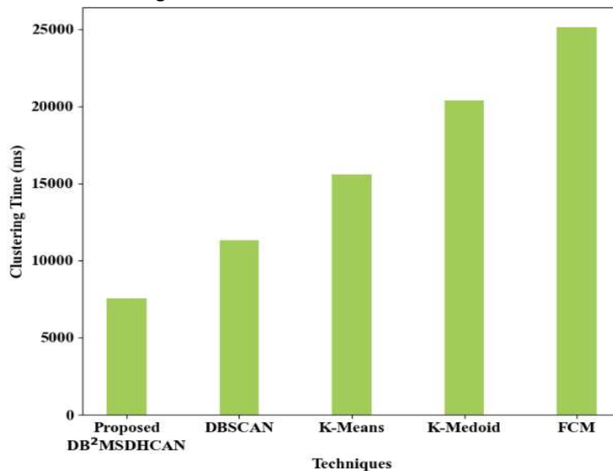
Figure 5: Clustering time validation
