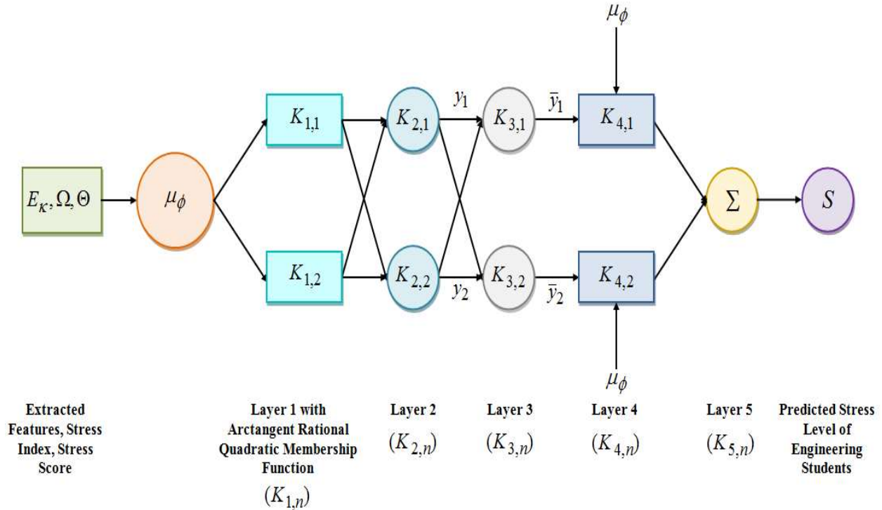
Figure 2: A 2 RQNFIS diagram
