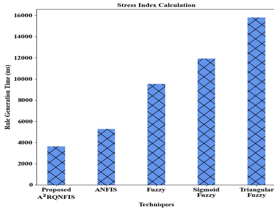
Figure 3: Rule generation time analysis
