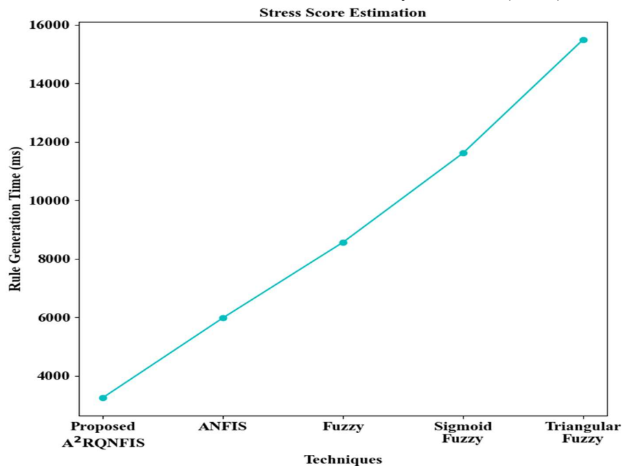
Figure 6: Graphical analysis of rule generation time
