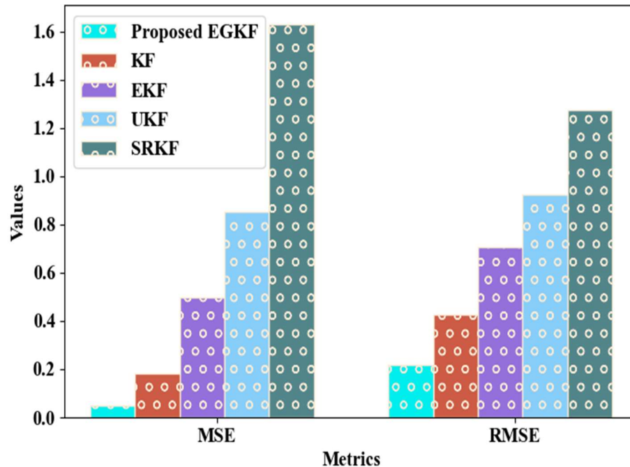
Figure 7: Comparative assessment of the proposed model
