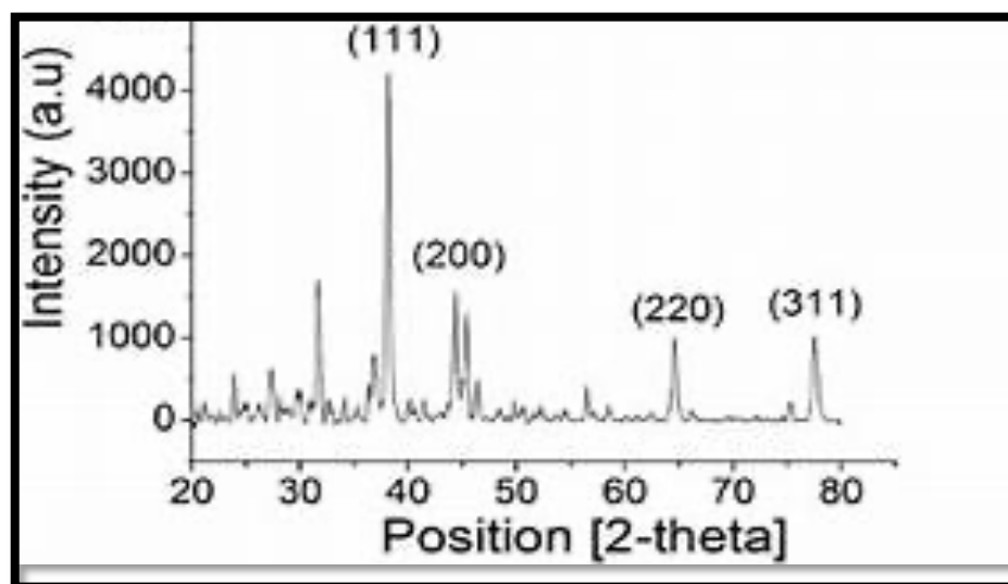
Fig 4.XRD pattern of nanoparticles present in leaf powder display peaks as 111, 200, 220, and 311are confirmative to crystallite points
